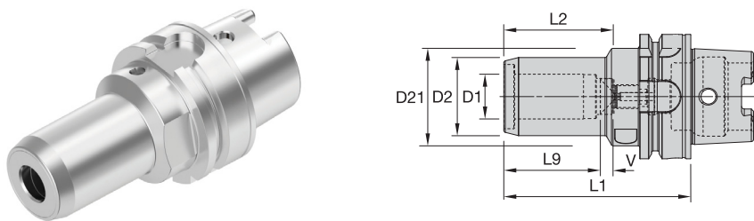
Hydraulic Chuck HSK63A • ML 1 Channel
