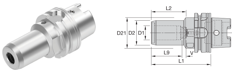
Hydraulic Chuck HSK63A • MQL 2 Channel
